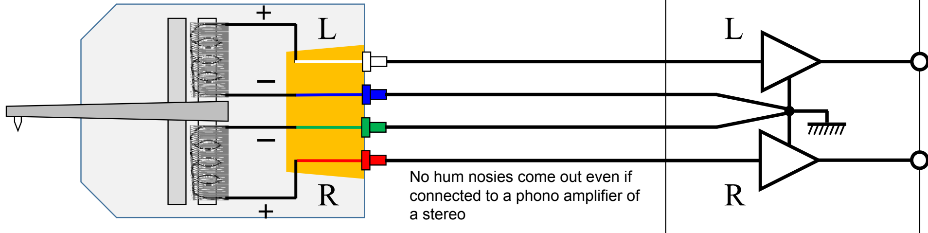
Dual Coil Type Monaural Cartridge, Phasemation PP-Mono, and so forth
