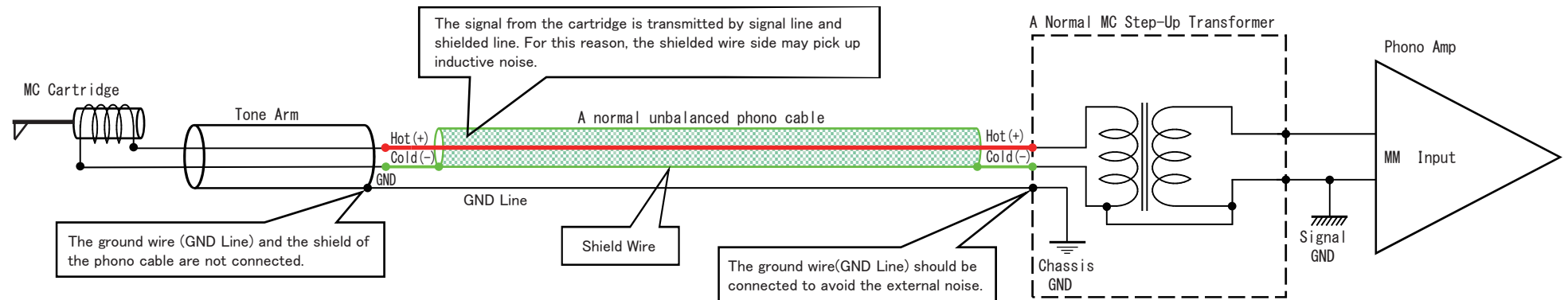
Fig 2:A Normal Phono Unbalanced Transmission
