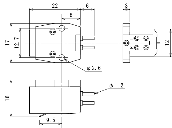
Dimensions figure(mm)
